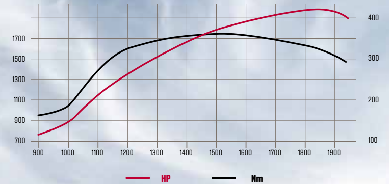
TORQUE IN NM, S396 AND S416
